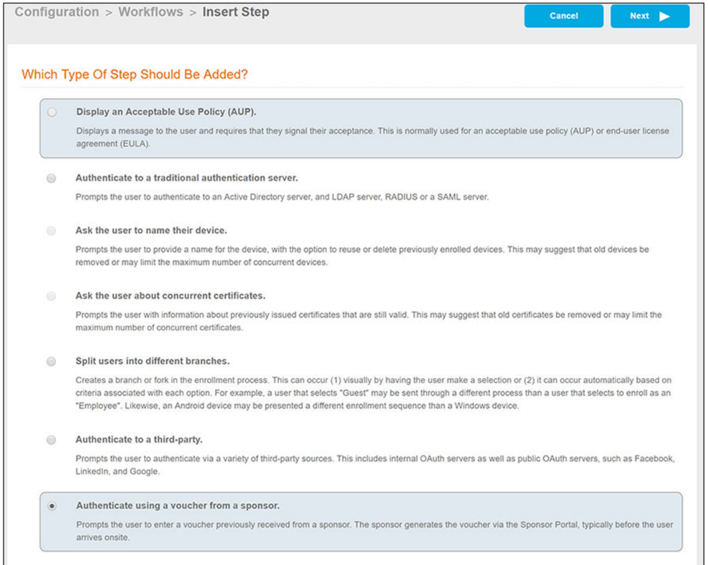
FIGURE 4 Using the "Authenticate using a voucher from a sponsor" Option in Your Alexa Workflow
